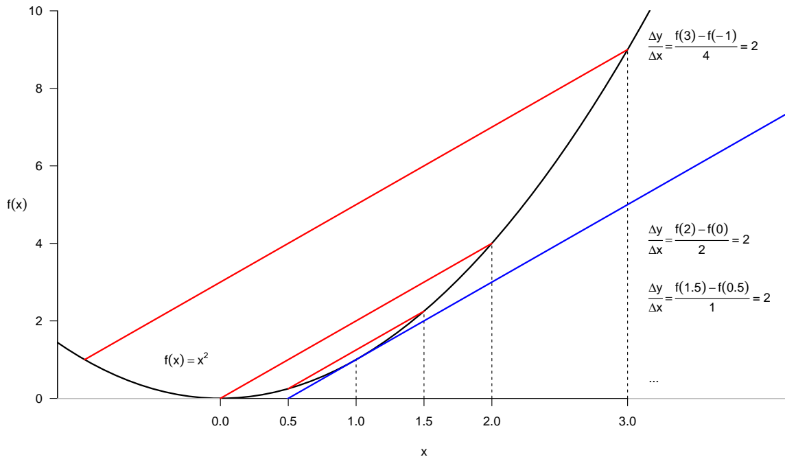
Figure 4: Approximation of Derivative via Two-Sided Numerical Approach
